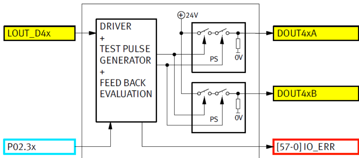
Figure 32: Block diagram of the two-channel safe outputs
