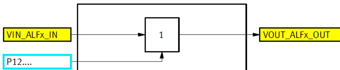
Figure 30: Block diagram, Advanced Logic Function
